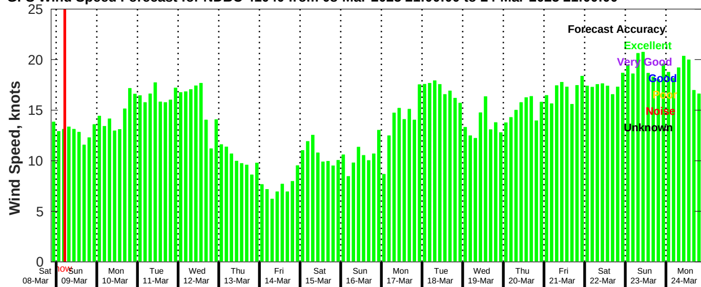
GFS Wind Speed Forecast for NDBC 41040 from 08-Mar-2025 21:00:00 to 24-Mar-2025 21:00:00
