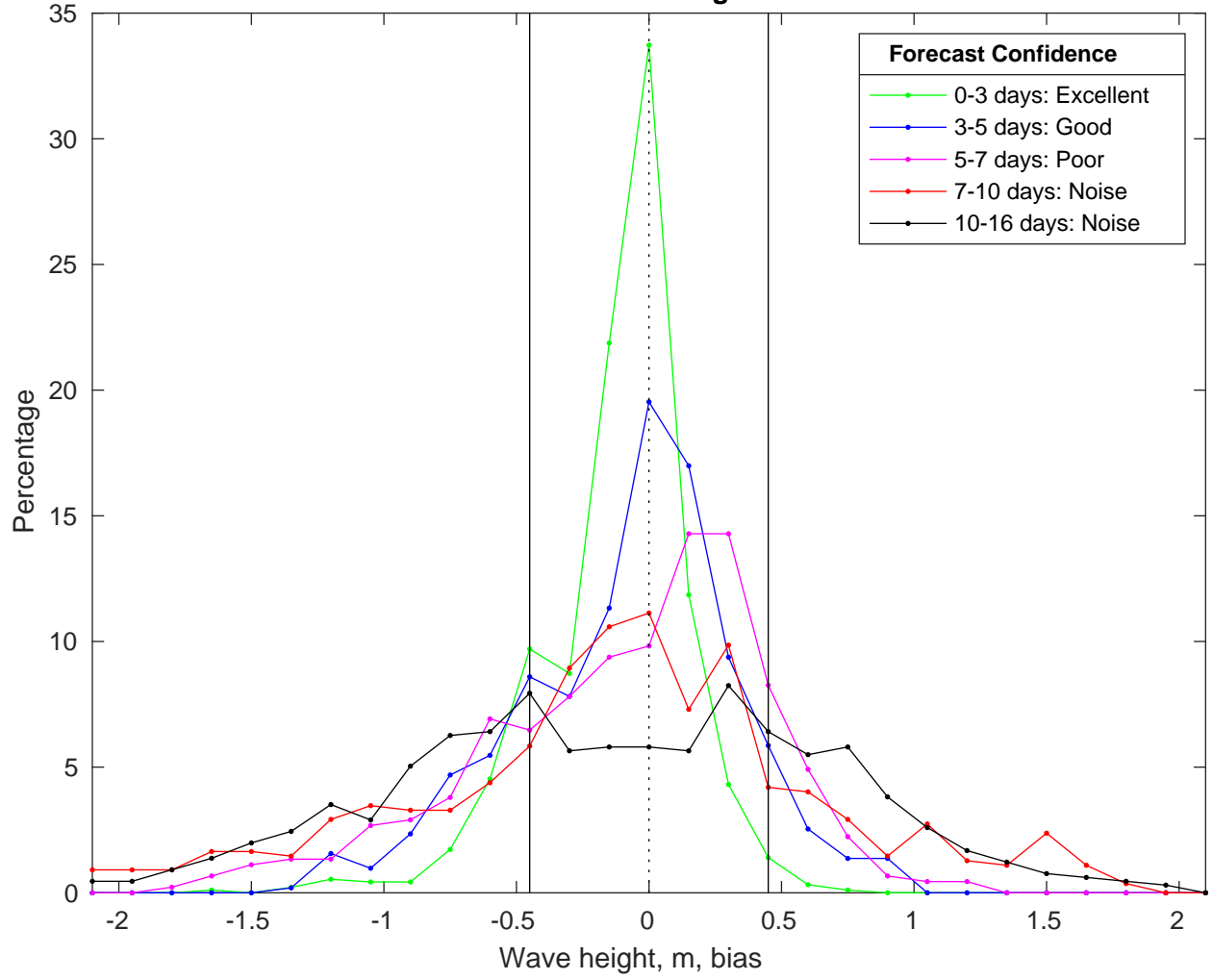
NDBC 42019 vs GFS Waves Bias Histogram: 09-Mar-2025
