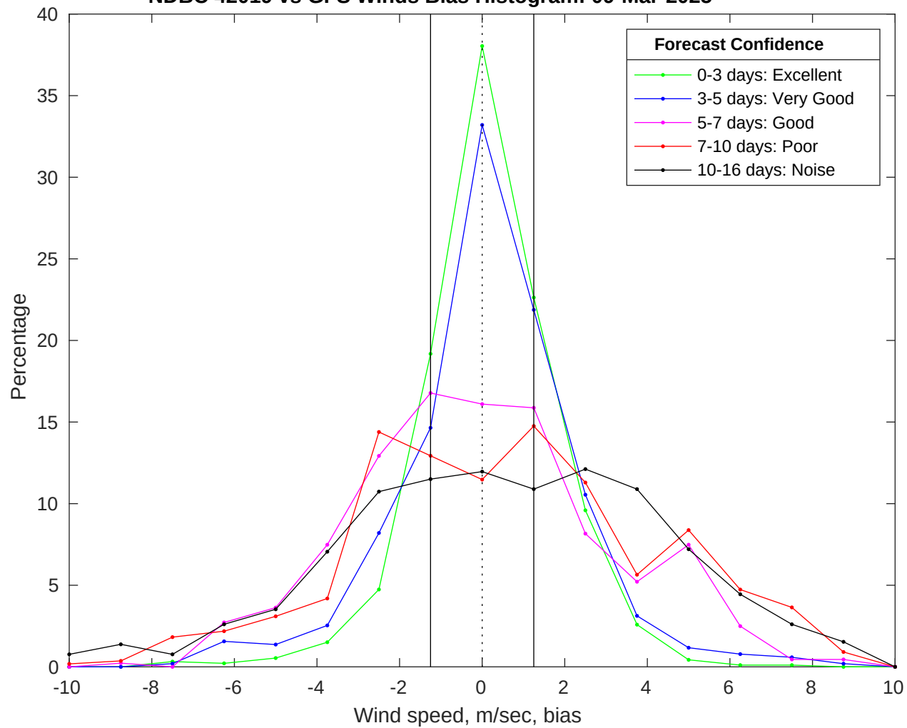
NDBC 42019 vs GFS Winds Bias Histogram: 09-Mar-2025
