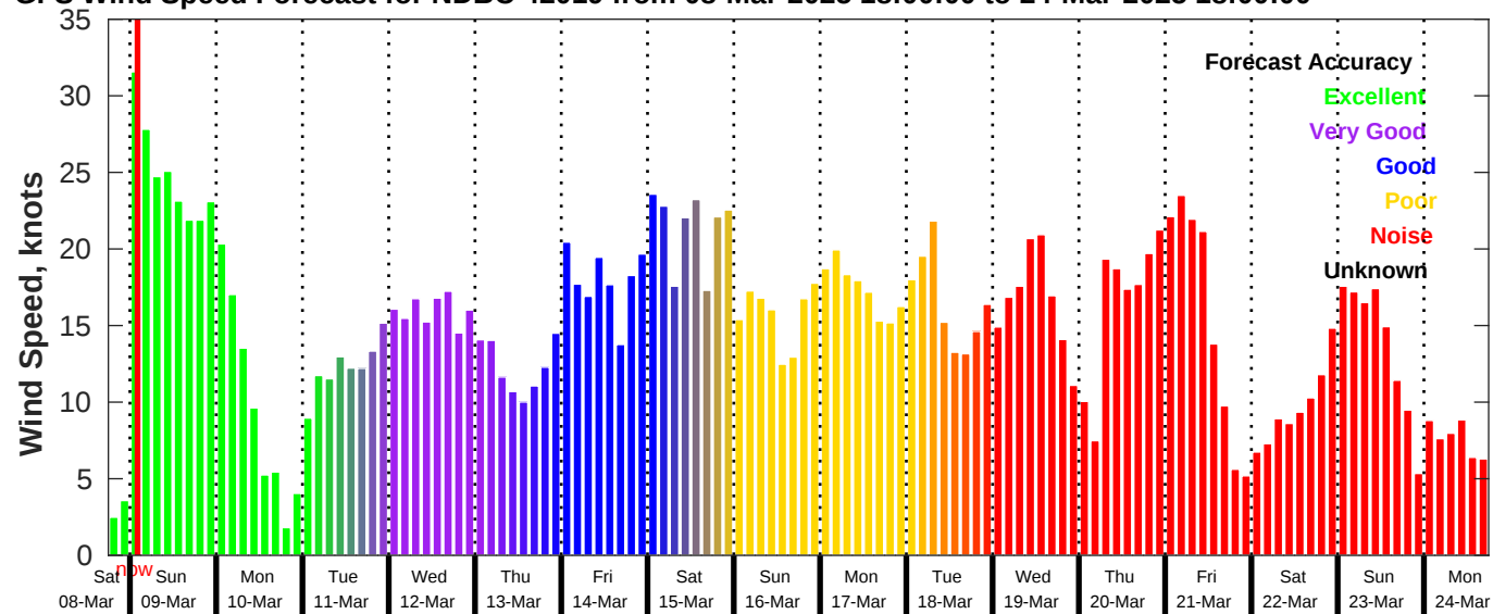
GFS Wind Speed Forecast for NDBC 42019 from 08-Mar-2025 18:00:00 to 24-Mar-2025 18:00:00
