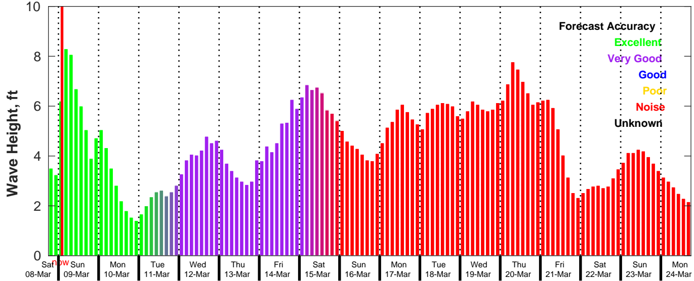
GFS Wave Forecast for NDBC 42020 from 08-Mar-2025 18:00:00 to 24-Mar-2025 18:00:00
