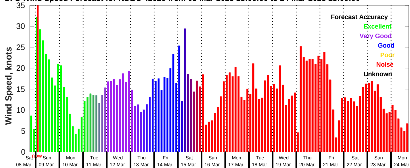
GFS Wind Speed Forecast for NDBC 42020 from 08-Mar-2025 18:00:00 to 24-Mar-2025 18:00:00
