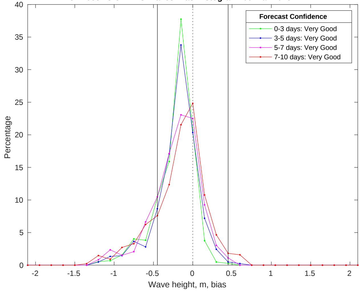
NDBC 42035 vs CMEMS Waves Bias Histogram: 09-Mar-2025
