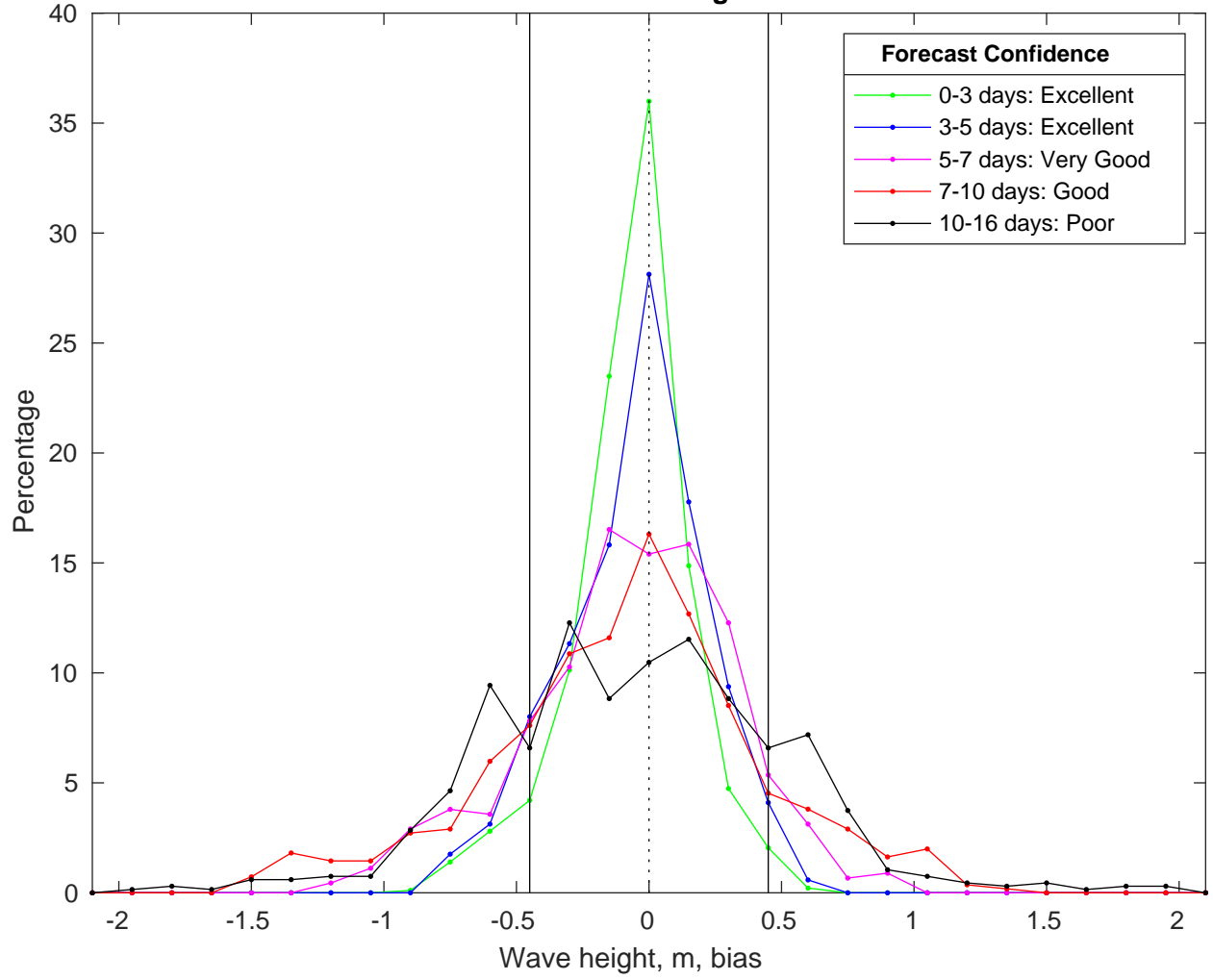
NDBC 42035 vs GFS Waves Bias Histogram: 09-Mar-2025
