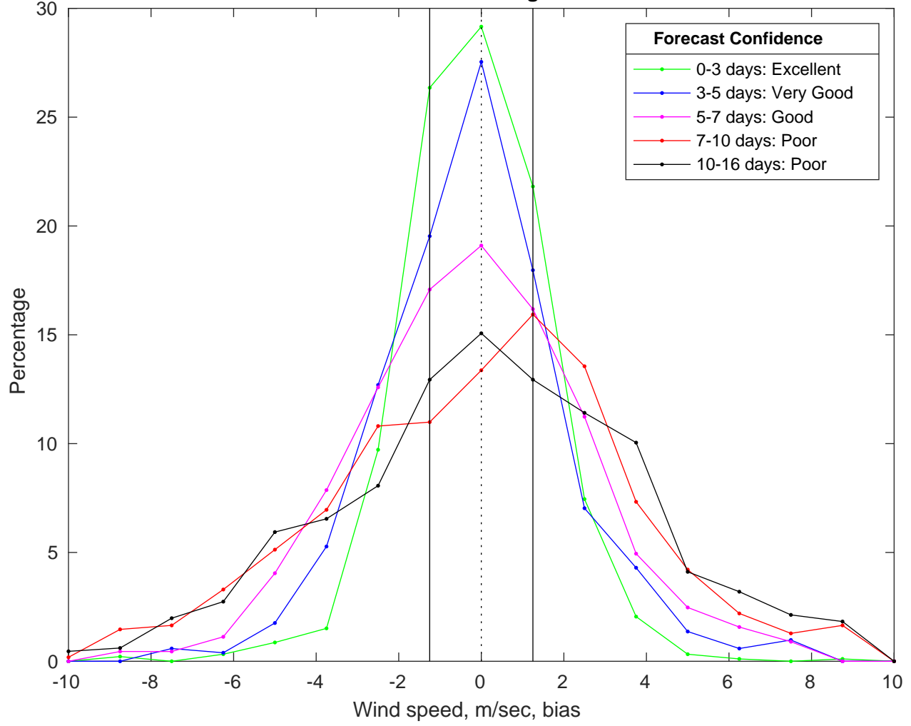
NDBC 42035 vs GFS Winds Bias Histogram: 09-Mar-2025
