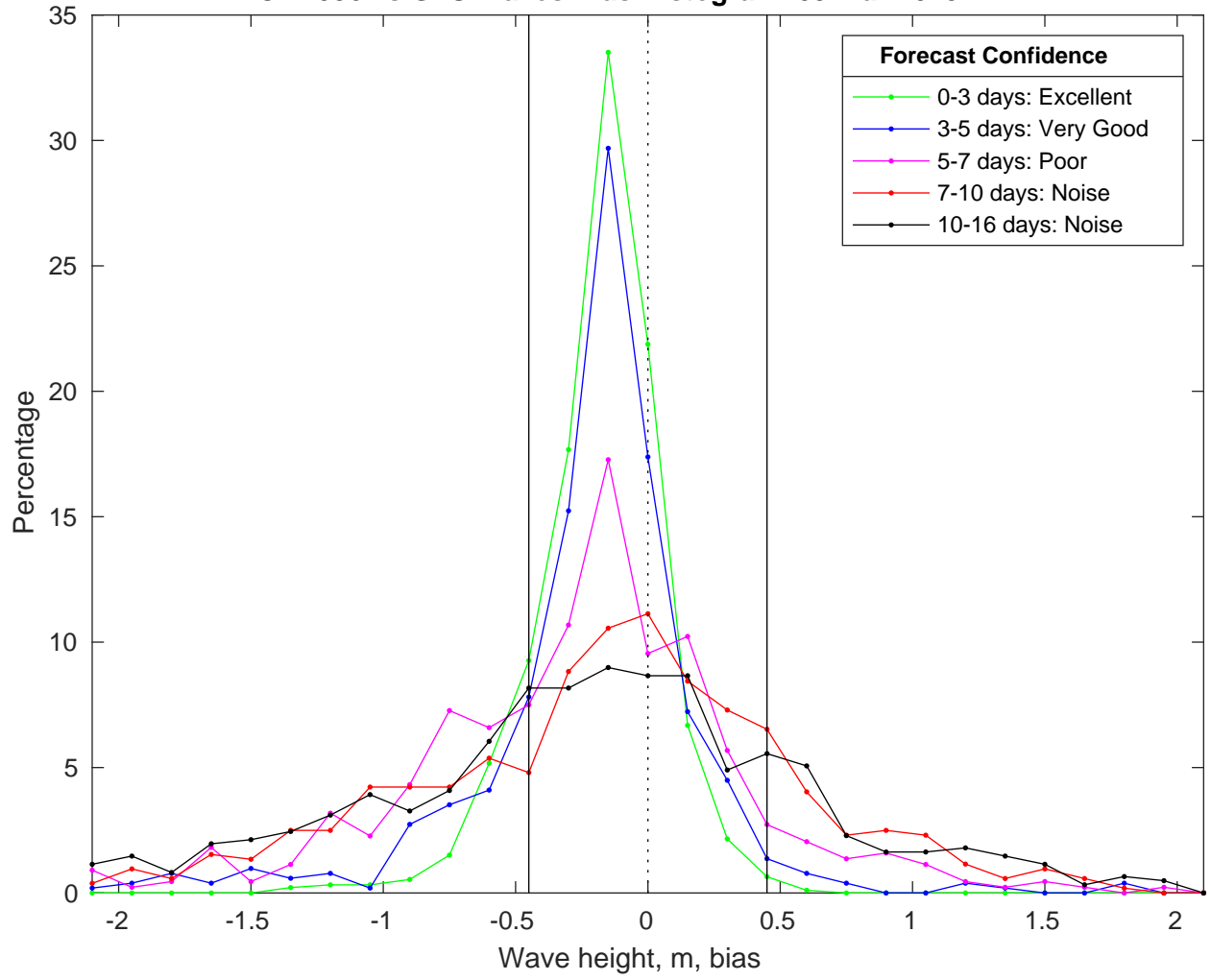
NDBC 42036 vs GFS Waves Bias Histogram: 09-Mar-2025
