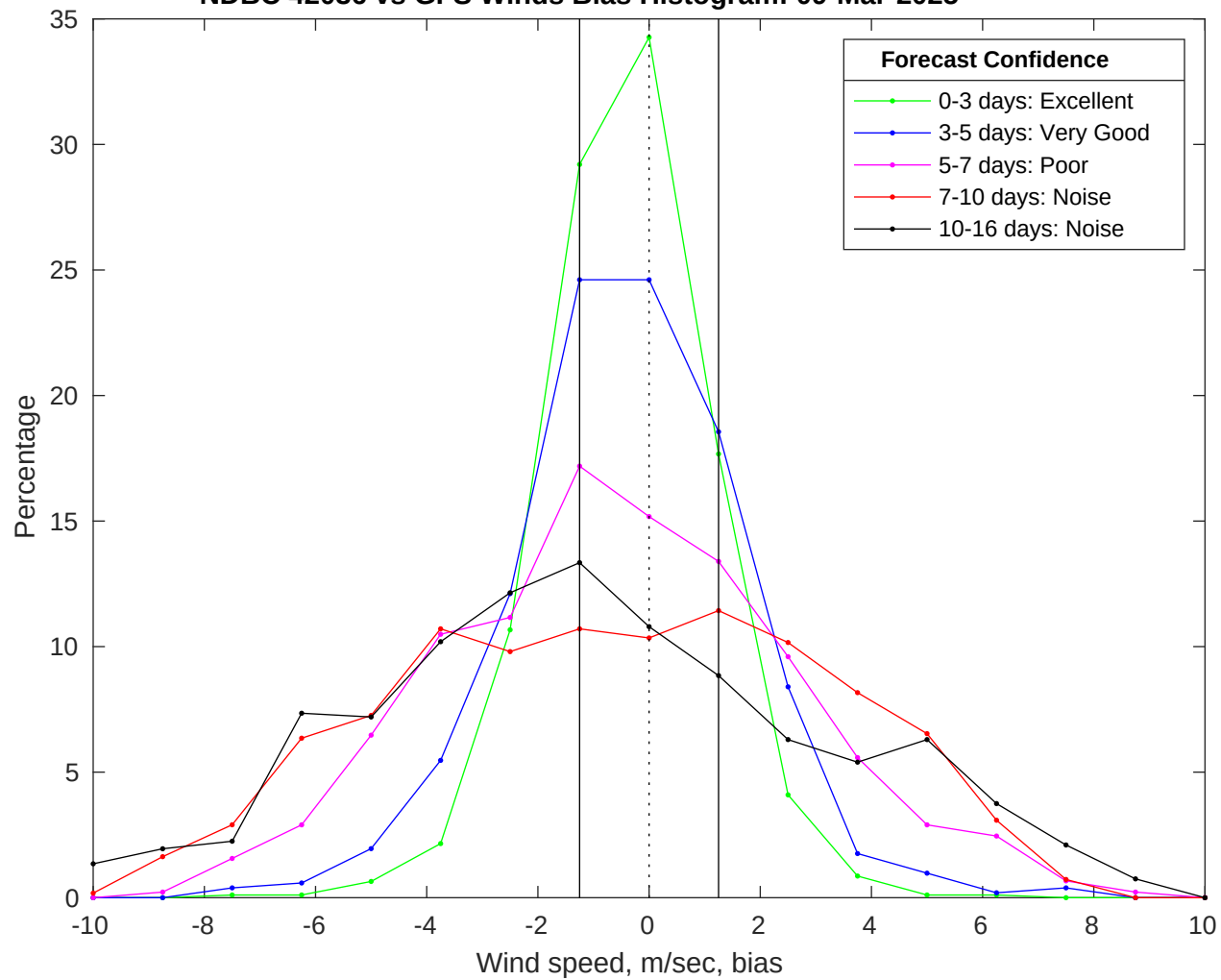
NDBC 42036 vs GFS Winds Bias Histogram: 09-Mar-2025
