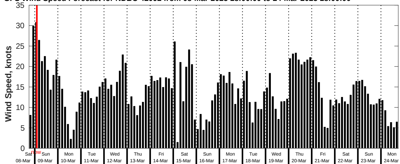
GFS Wind Speed Forecast for NDBC 42092 from 08-Mar-2025 18:00:00 to 24-Mar-2025 18:00:00
