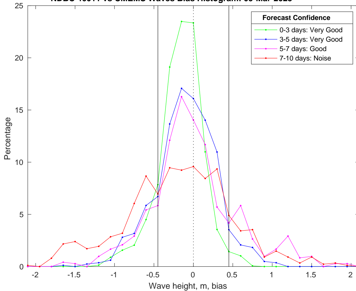
NDBC 46011 vs CMEMS Waves Bias Histogram: 09-Mar-2025
