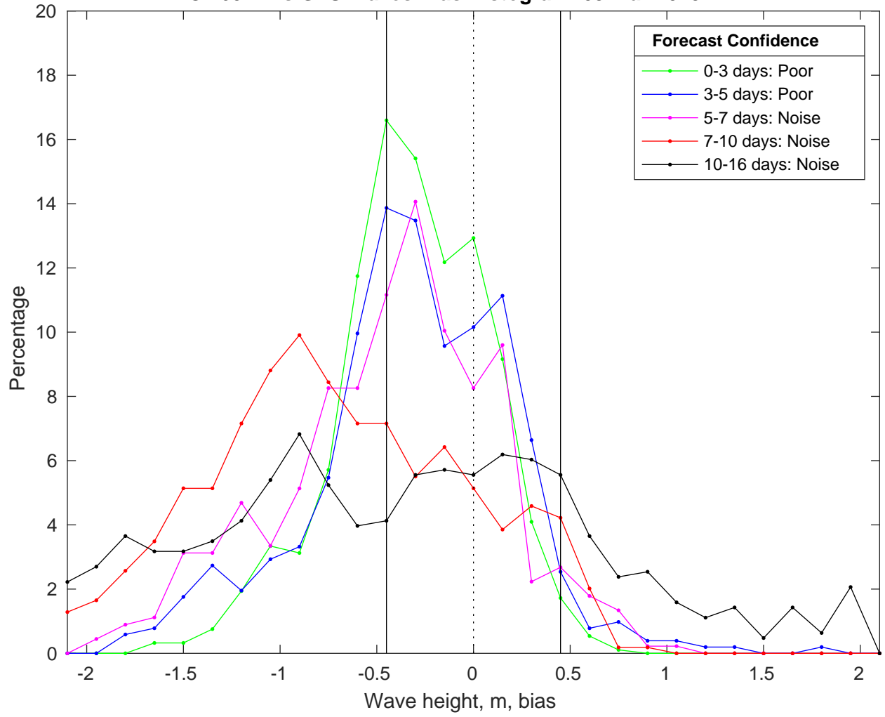
NDBC 46011 vs GFS Waves Bias Histogram: 09-Mar-2025
