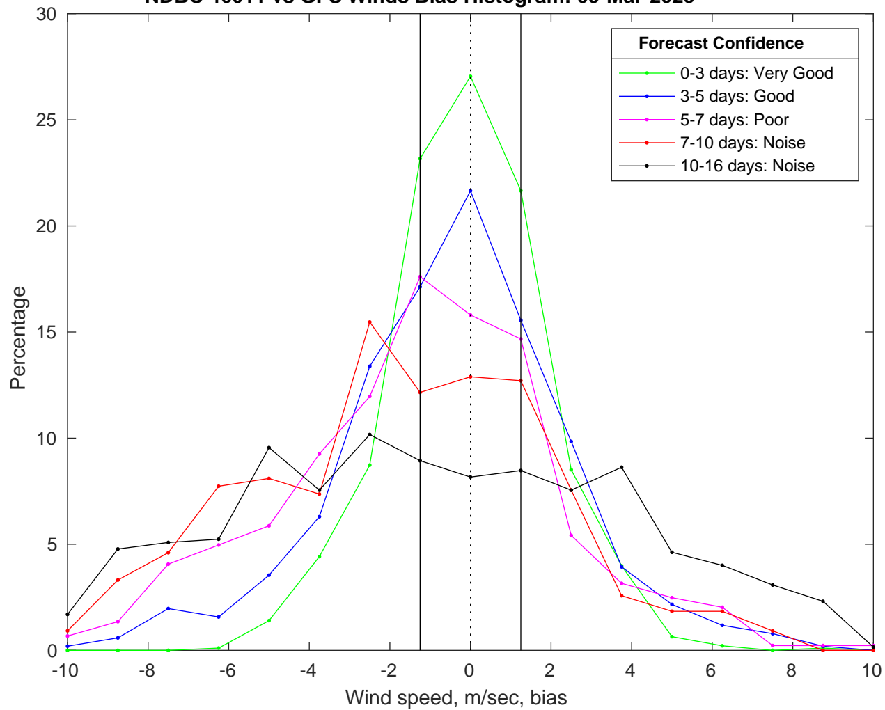
NDBC 46011 vs GFS Winds Bias Histogram: 09-Mar-2025
