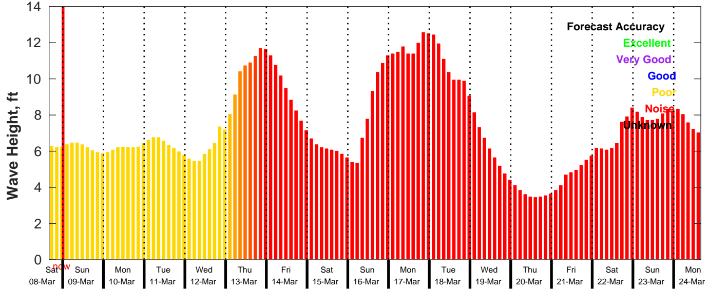
GFS Wave Forecast for NDBC 46011 from 08-Mar-2025 16:00:00 to 24-Mar-2025 16:00:00
