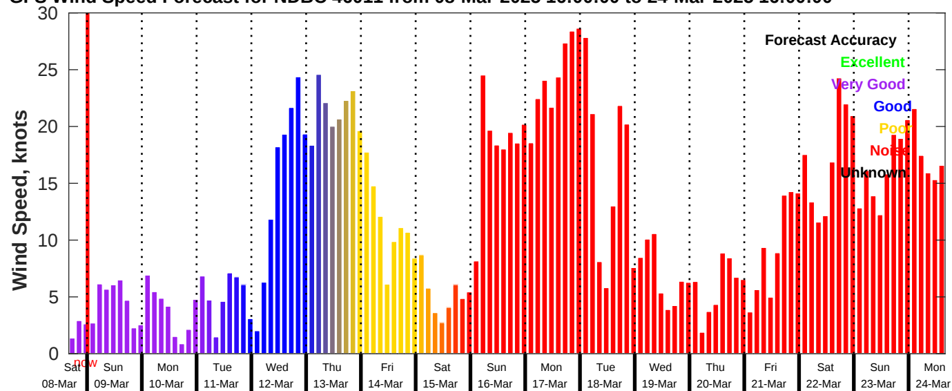
GFS Wind Speed Forecast for NDBC 46011 from 08-Mar-2025 16:00:00 to 24-Mar-2025 16:00:00
