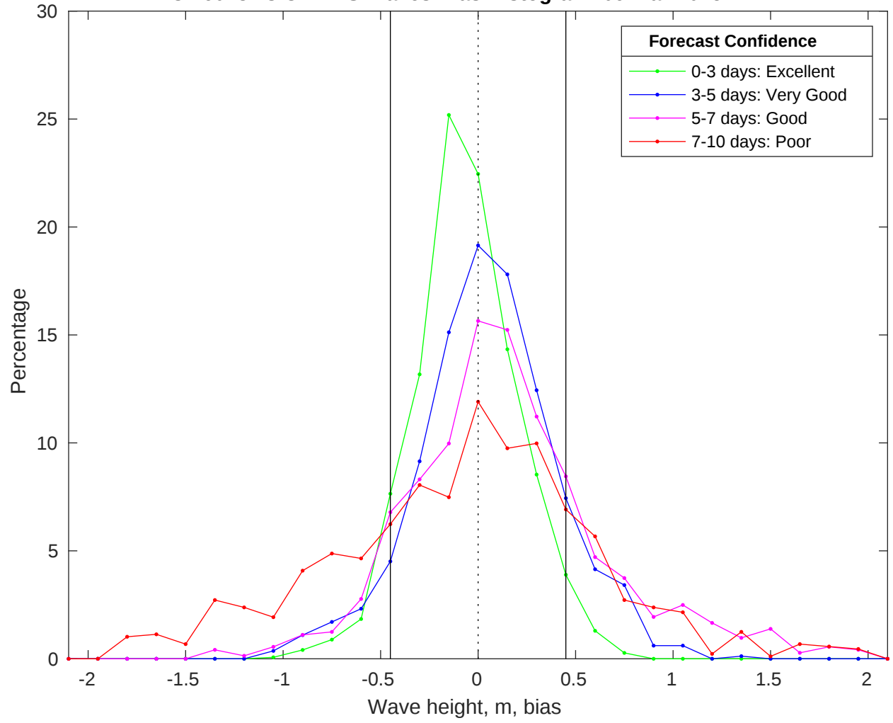
NDBC 46028 vs CMEMS Waves Bias Histogram: 09-Mar-2025
