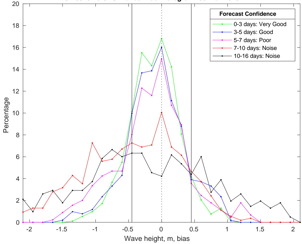
NDBC 46028 vs GFS Waves Bias Histogram: 09-Mar-2025
