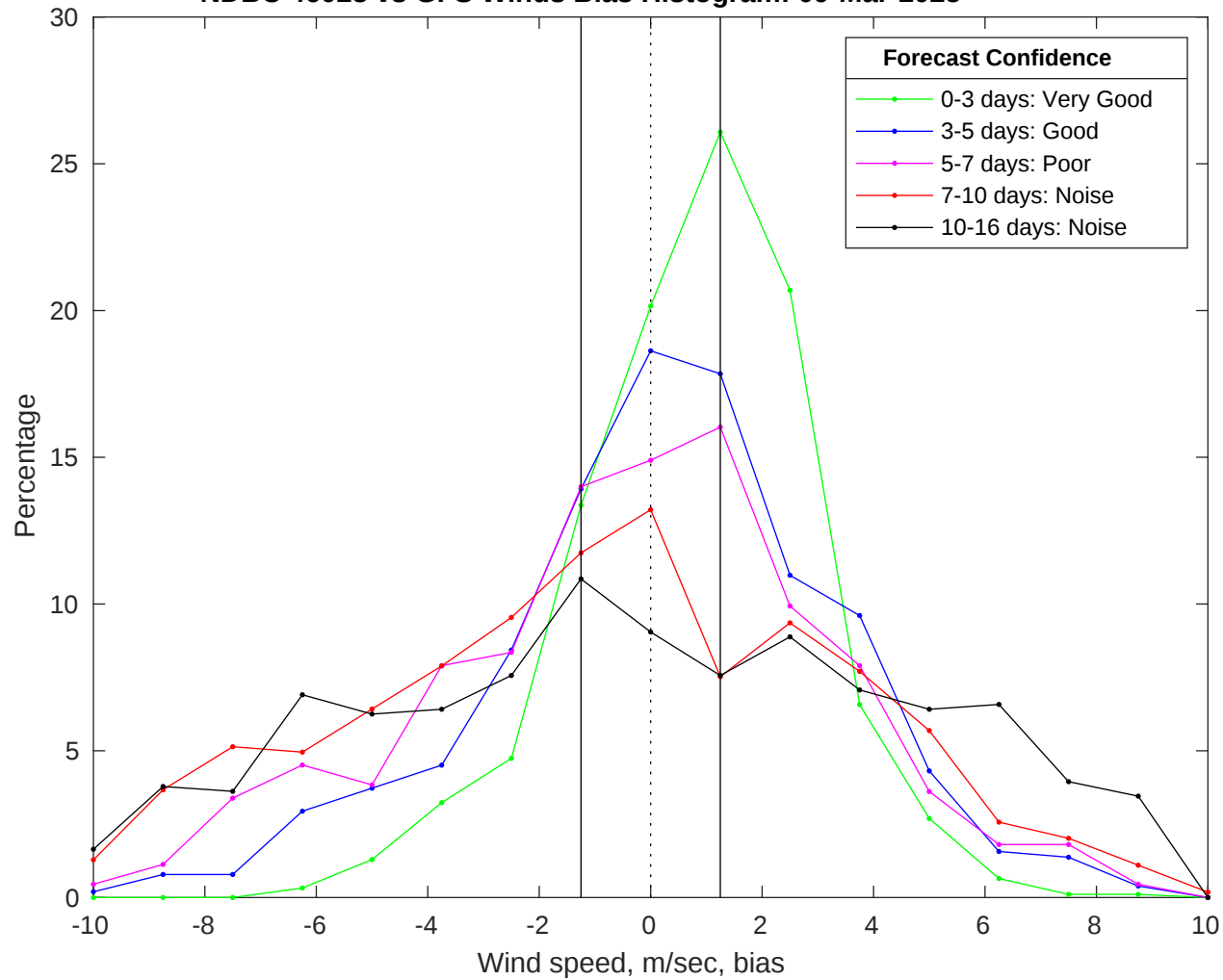
NDBC 46028 vs GFS Winds Bias Histogram: 09-Mar-2025
