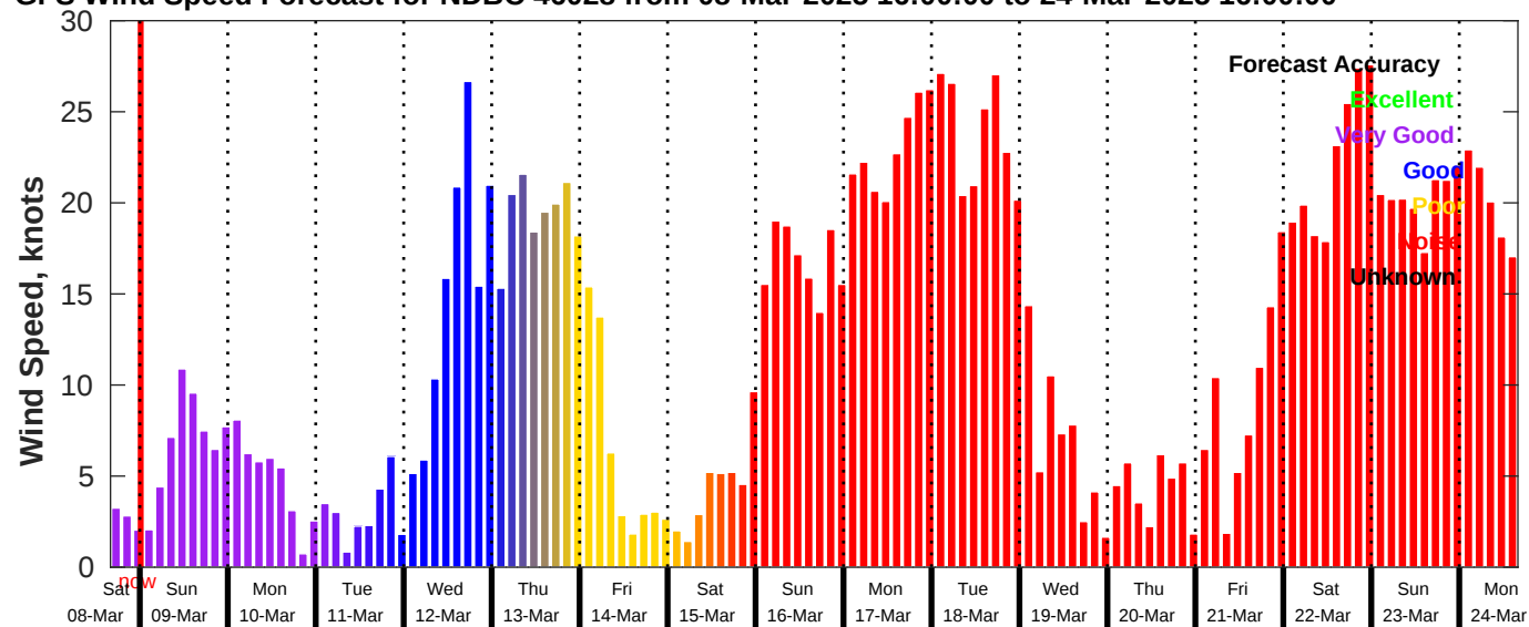
GFS Wind Speed Forecast for NDBC 46028 from 08-Mar-2025 16:00:00 to 24-Mar-2025 16:00:00
