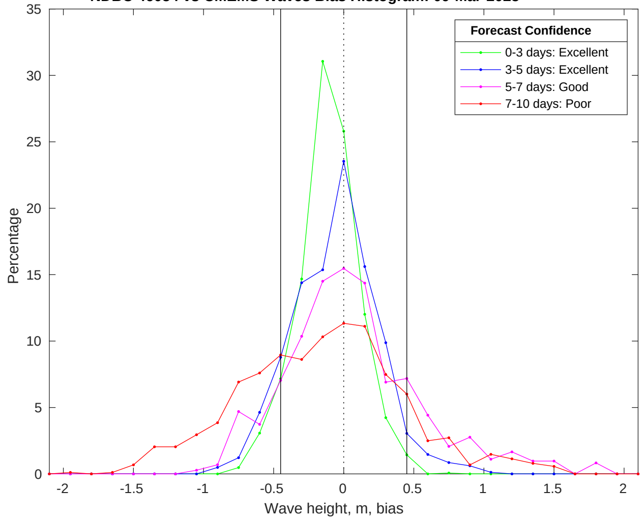
NDBC 46054 vs CMEMS Waves Bias Histogram: 09-Mar-2025
