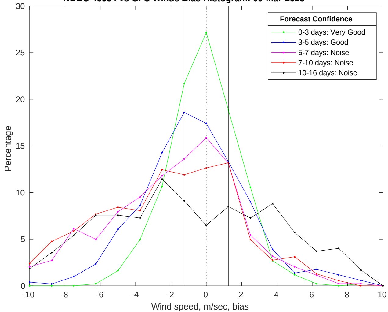
NDBC 46054 vs GFS Winds Bias Histogram: 09-Mar-2025
