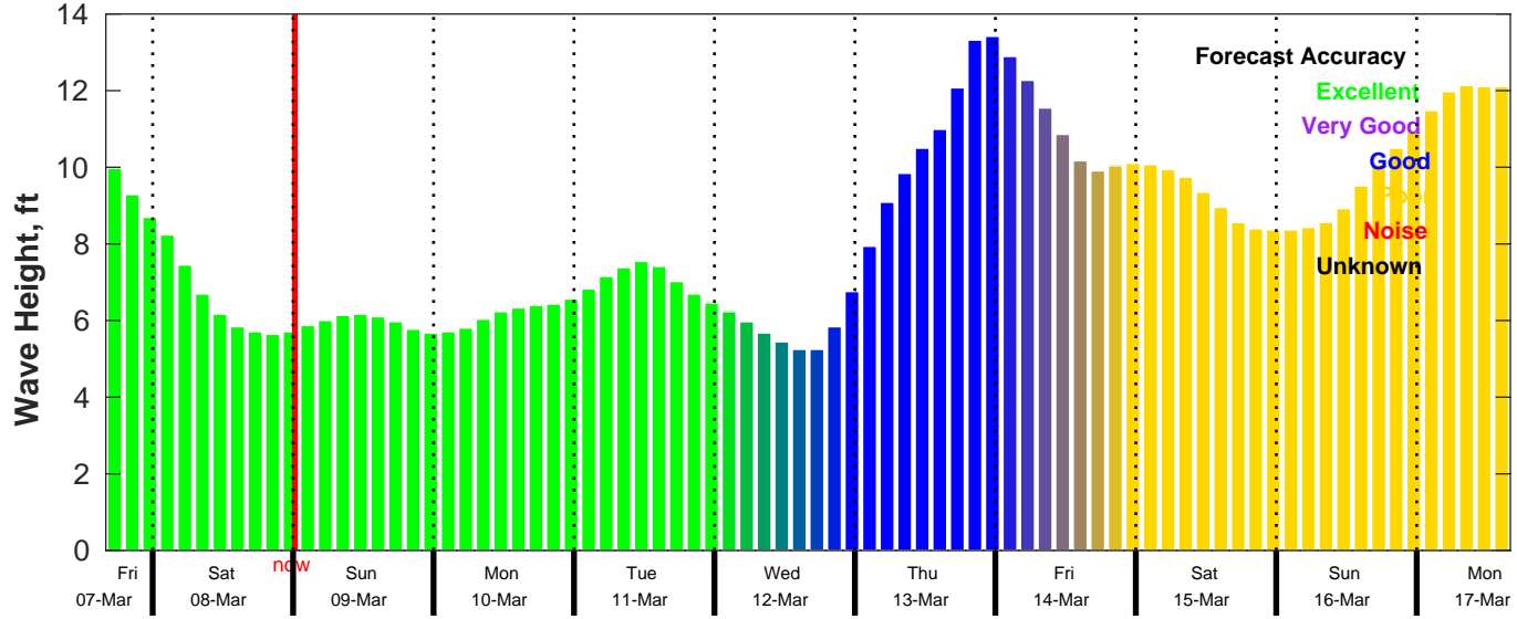
CMEMS Wave Forecast for NDBC 46054 from 07-Mar-2025 16:00:00 to 17-Mar-2025 16:00:00
