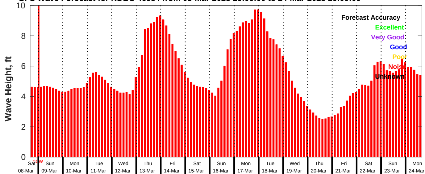
GFS Wave Forecast for NDBC 46054 from 08-Mar-2025 16:00:00 to 24-Mar-2025 16:00:00
