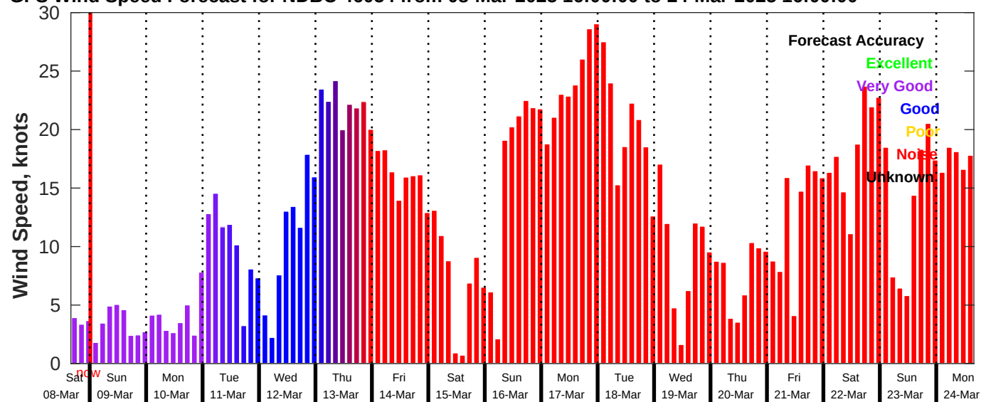
GFS Wind Speed Forecast for NDBC 46054 from 08-Mar-2025 16:00:00 to 24-Mar-2025 16:00:00
