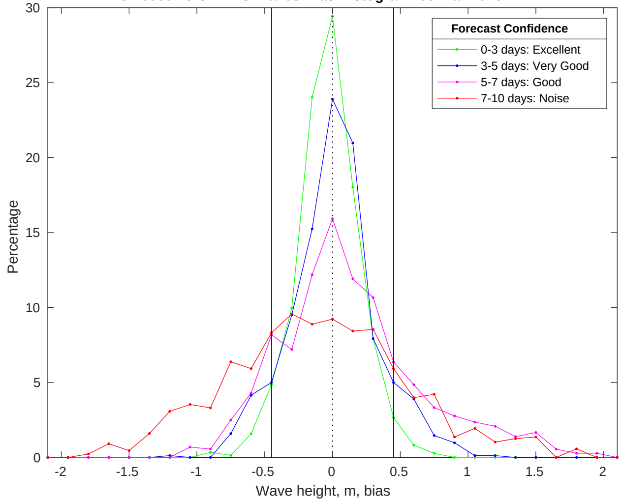
NDBC 46069 vs CMEMS Waves Bias Histogram: 09-Mar-2025
