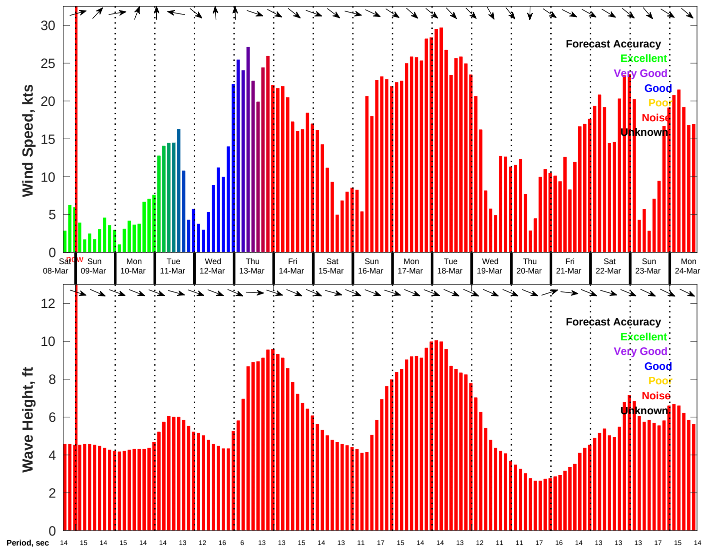
Wind & Wave Forecast for NDBC 46069 from 08-Mar-2025 16:00:00 to 24-Mar-2025 16:00:00
