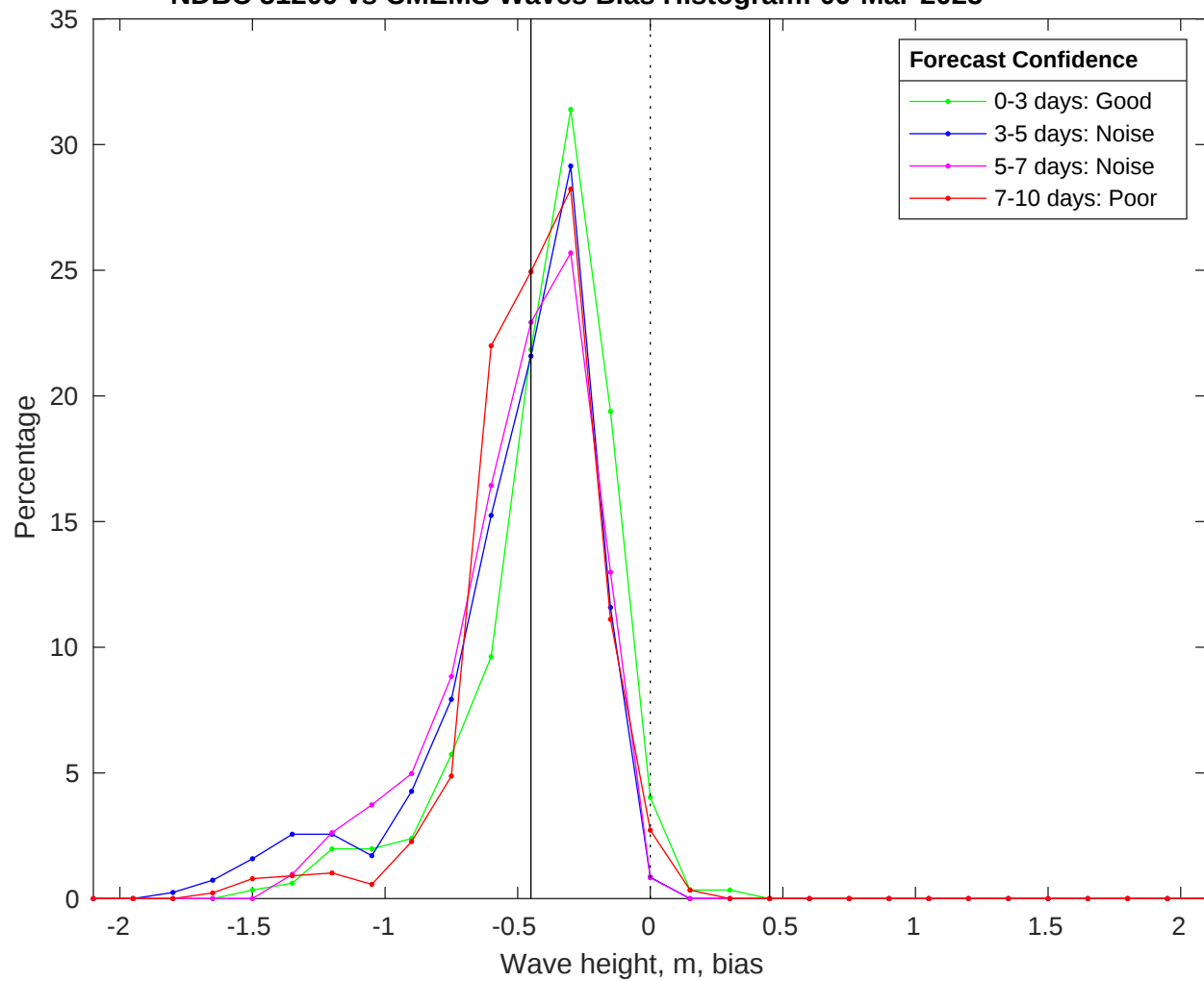
NDBC 51209 vs CMEMS Waves Bias Histogram: 09-Mar-2025
