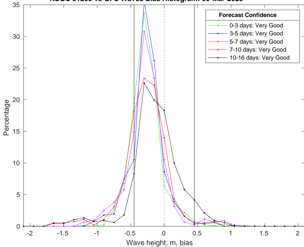
NDBC 51209 vs GFS Waves Bias Histogram: 09-Mar-2025
