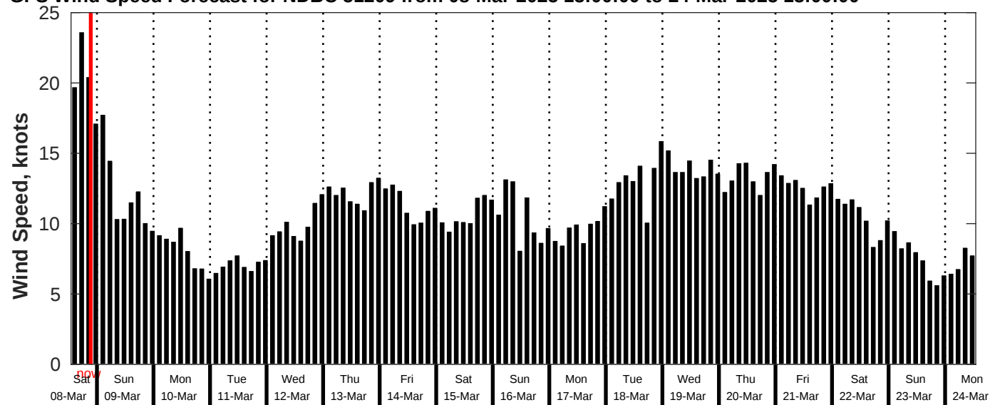
GFS Wind Speed Forecast for NDBC 51209 from 08-Mar-2025 13:00:00 to 24-Mar-2025 13:00:00
