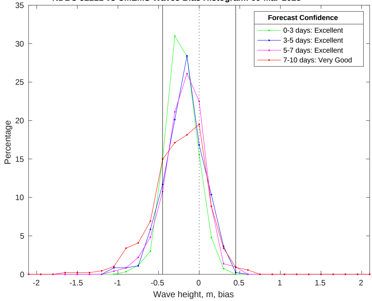
NDBC 52211 vs CMEMS Waves Bias Histogram: 09-Mar-2025
