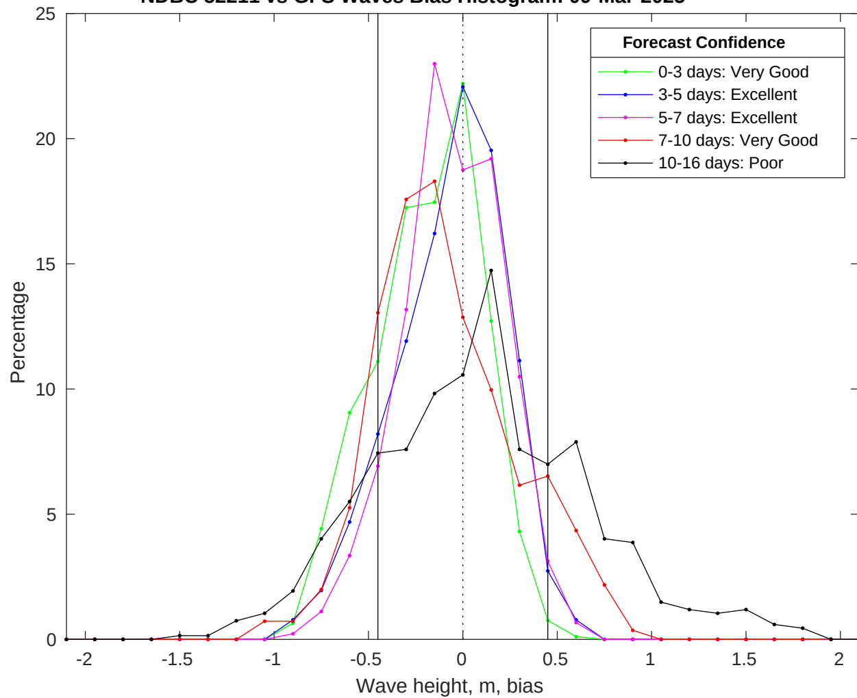
NDBC 52211 vs GFS Waves Bias Histogram: 09-Mar-2025
