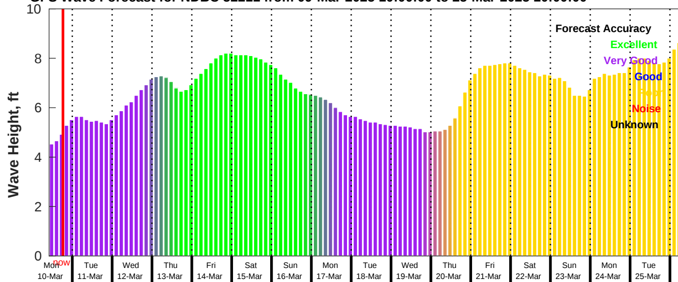
GFS Wave Forecast for NDBC 52211 from 09-Mar-2025 10:00:00 to 25-Mar-2025 10:00:00
