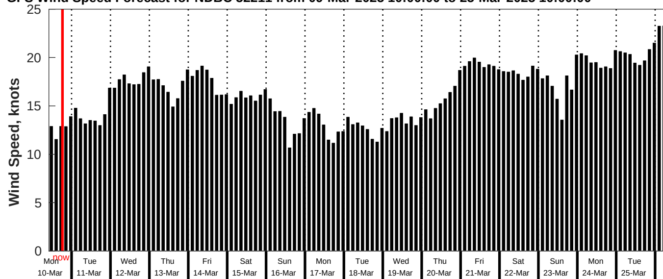
GFS Wind Speed Forecast for NDBC 52211 from 09-Mar-2025 10:00:00 to 25-Mar-2025 10:00:00
