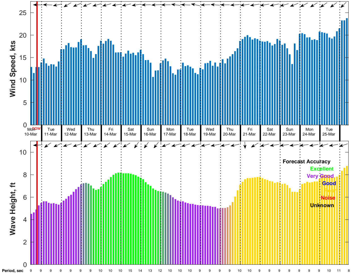
Wind & Wave Forecast for NDBC 52211 from 09-Mar-2025 10:00:00 to 25-Mar-2025 10:00:00
