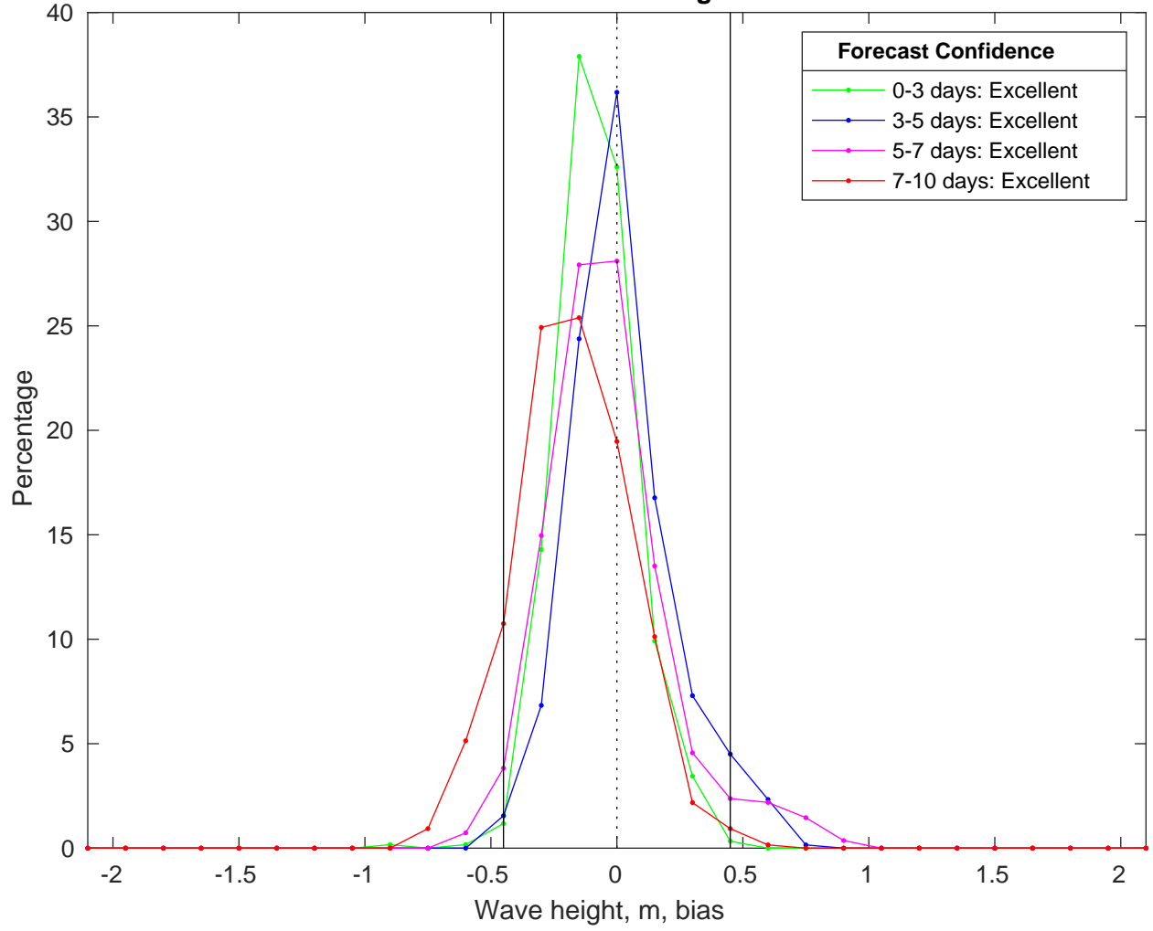
NDBC 52212 vs CMEMS Waves Bias Histogram: 09-Mar-2025
