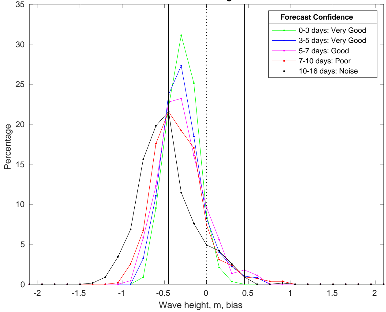
NDBC 52212 vs GFS Waves Bias Histogram: 09-Mar-2025
