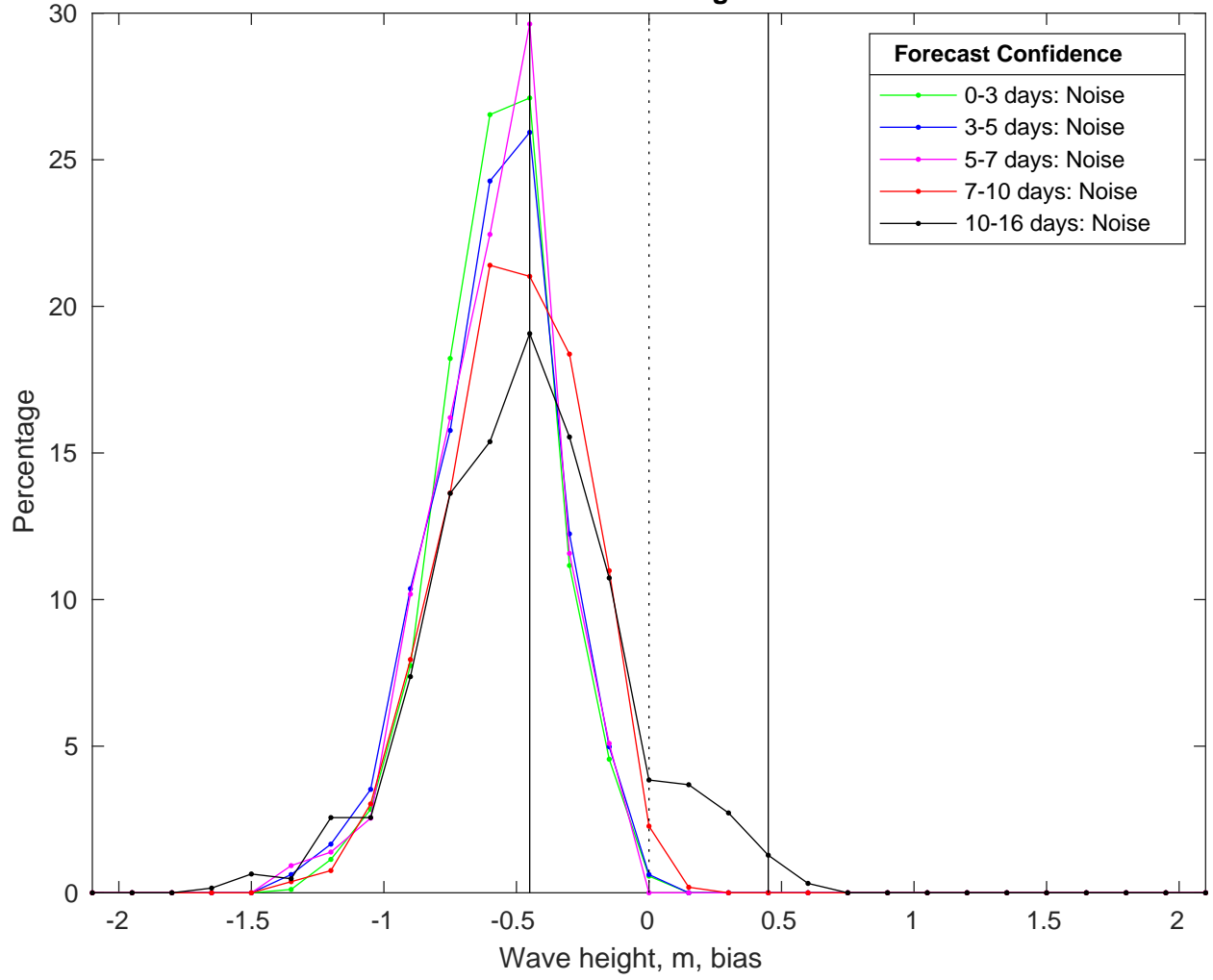
NDBC 52213 vs GFS Waves Bias Histogram: 09-Mar-2025
