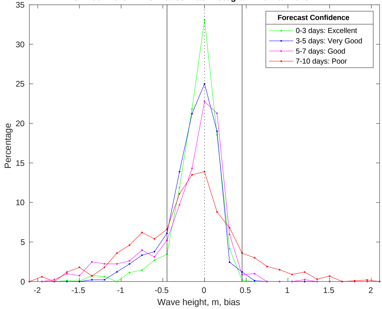
NDBC 41004 vs CMEMS Waves Bias Histogram: 10-Mar-2025
