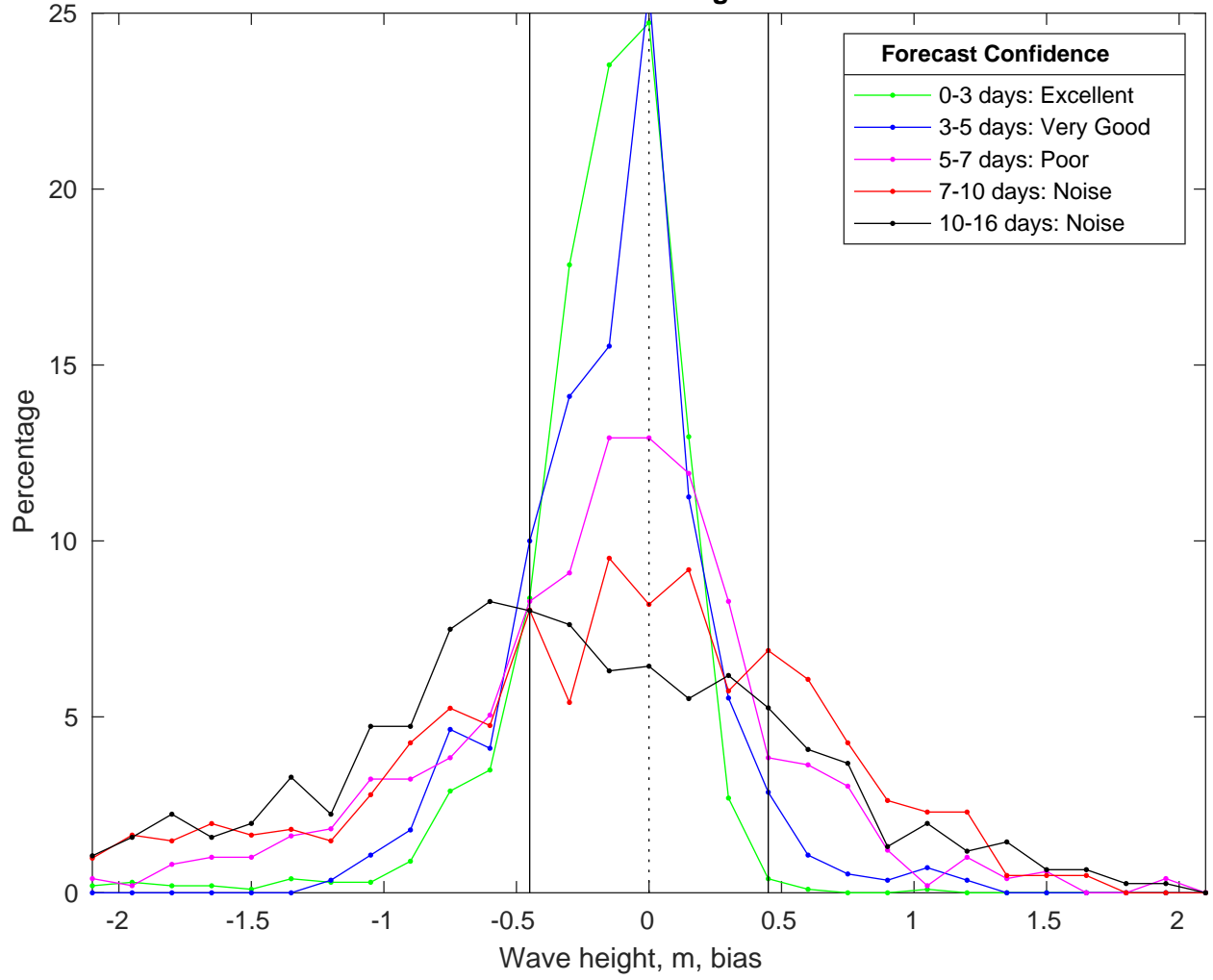
NDBC 41004 vs GFS Waves Bias Histogram: 10-Mar-2025
