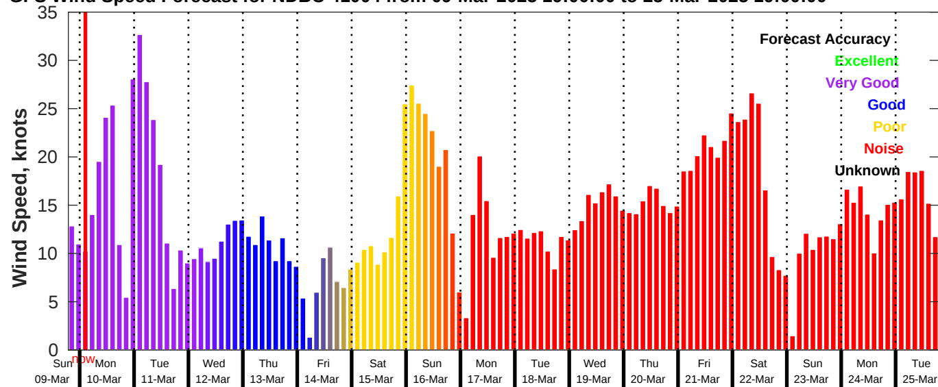
GFS Wind Speed Forecast for NDBC 41004 from 09-Mar-2025 19:00:00 to 25-Mar-2025 19:00:00
