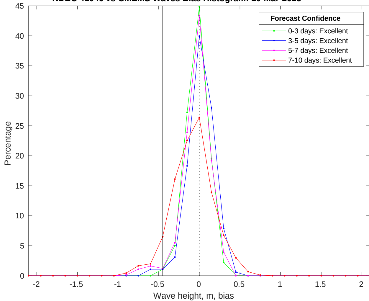
NDBC 41040 vs CMEMS Waves Bias Histogram: 10-Mar-2025
