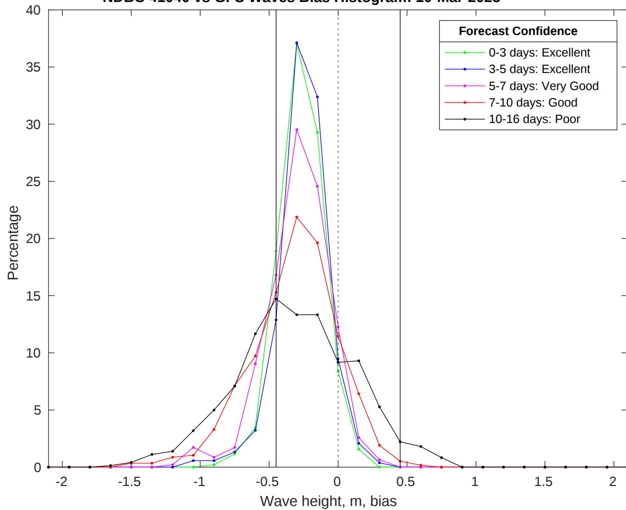
NDBC 41040 vs GFS Waves Bias Histogram: 10-Mar-2025
