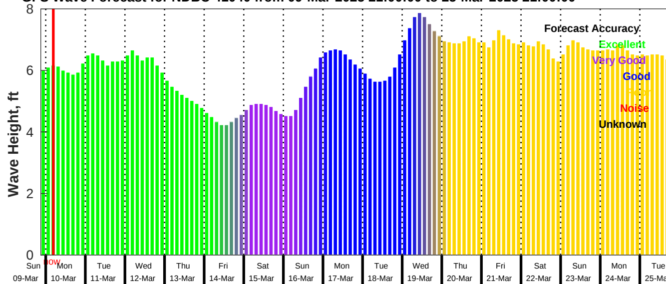
GFS Wave Forecast for NDBC 41040 from 09-Mar-2025 21:00:00 to 25-Mar-2025 21:00:00
