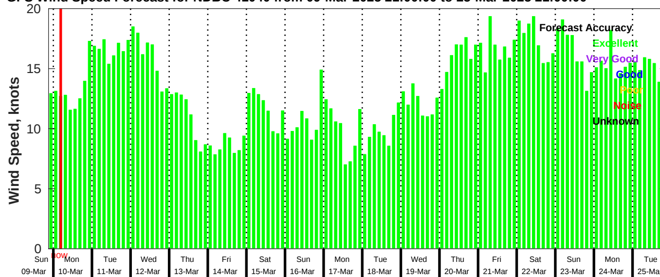
GFS Wind Speed Forecast for NDBC 41040 from 09-Mar-2025 21:00:00 to 25-Mar-2025 21:00:00
