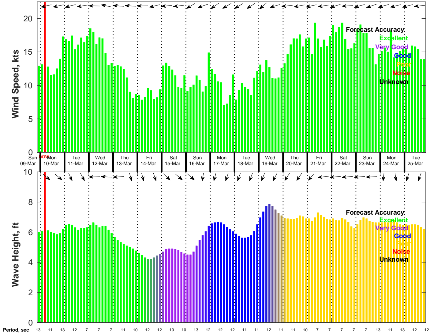
Wind & Wave Forecast for NDBC 41040 from 09-Mar-2025 21:00:00 to 25-Mar-2025 21:00:00
