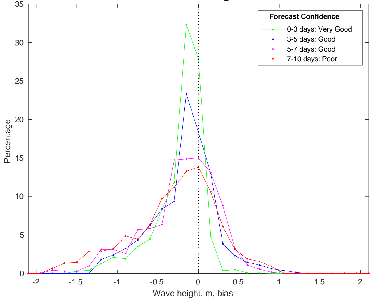
NDBC 42019 vs CMEMS Waves Bias Histogram: 10-Mar-2025
