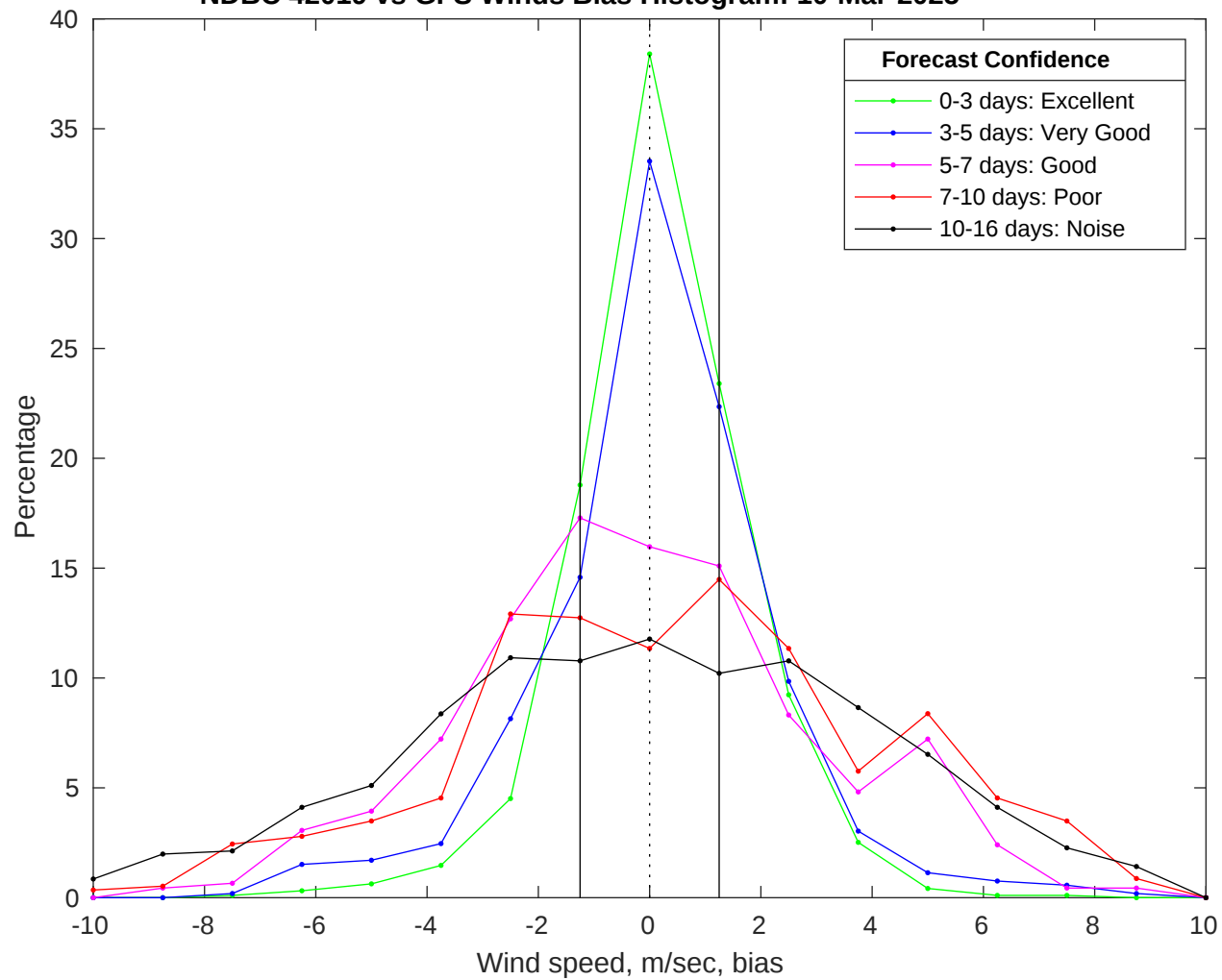
NDBC 42019 vs GFS Winds Bias Histogram: 10-Mar-2025
