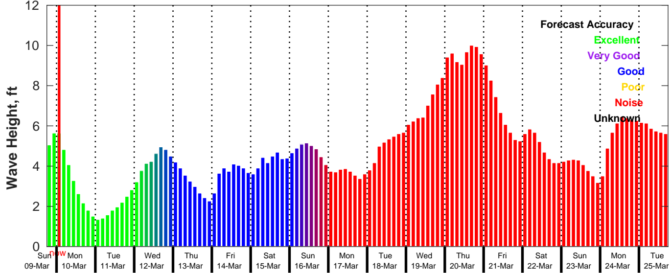
GFS Wave Forecast for NDBC 42019 from 09-Mar-2025 18:00:00 to 25-Mar-2025 18:00:00
